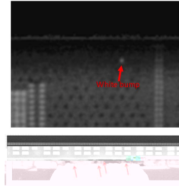
Figure 4: White bump scanning picture and bump cross-section after 20X reflow
